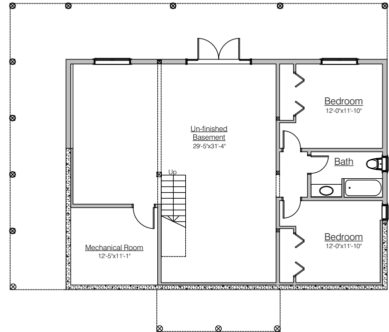
Basement 1518 Sq. Ft.
