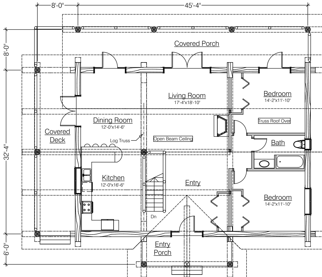
Main Floor Plan 1518 Sq. Ft.
