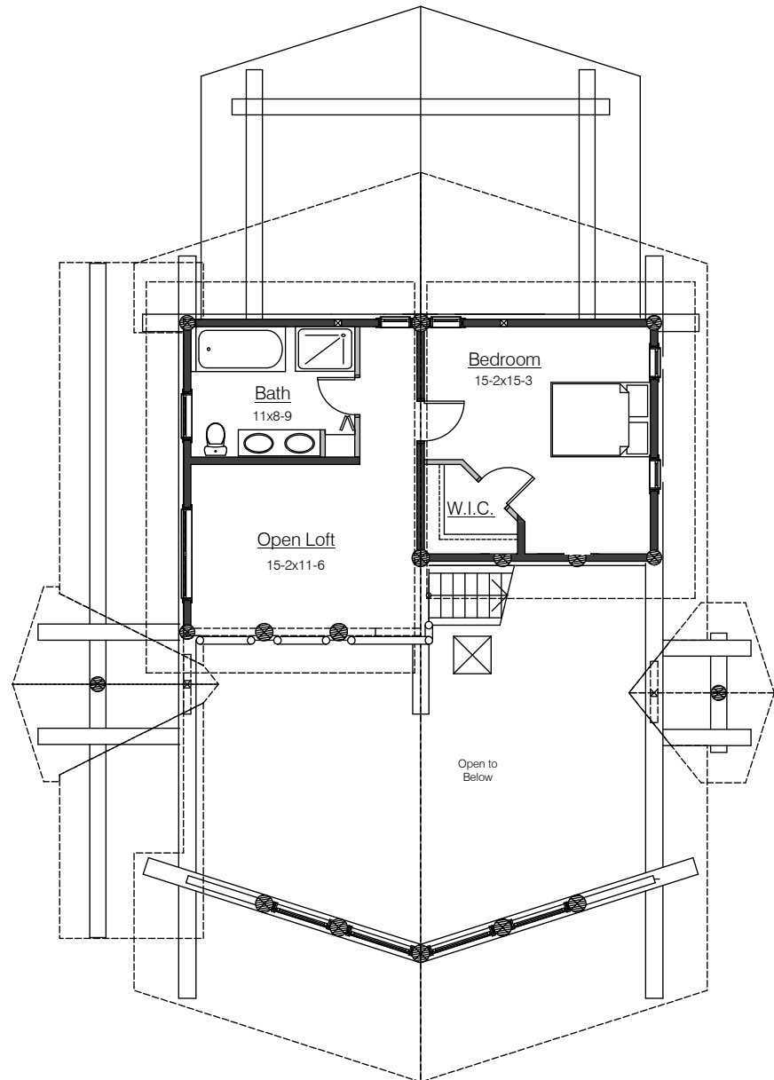
Loft Floor Plan 598 Sq. Ft. (Over 6' Headroom)
