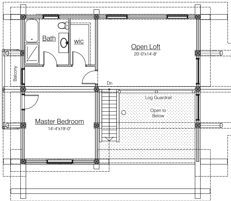
Loft Floor Plan 771 Sq. Ft. (Over 6' Headroom)
