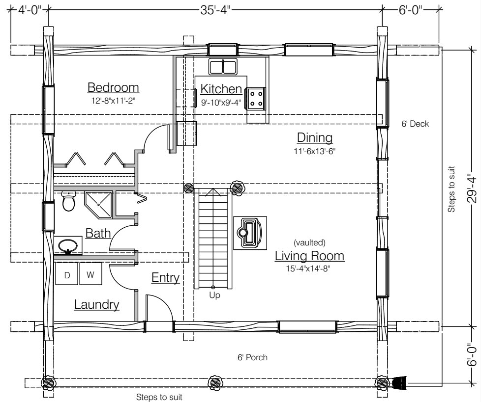
Main Floor Plan 1080 Sq. Ft.
